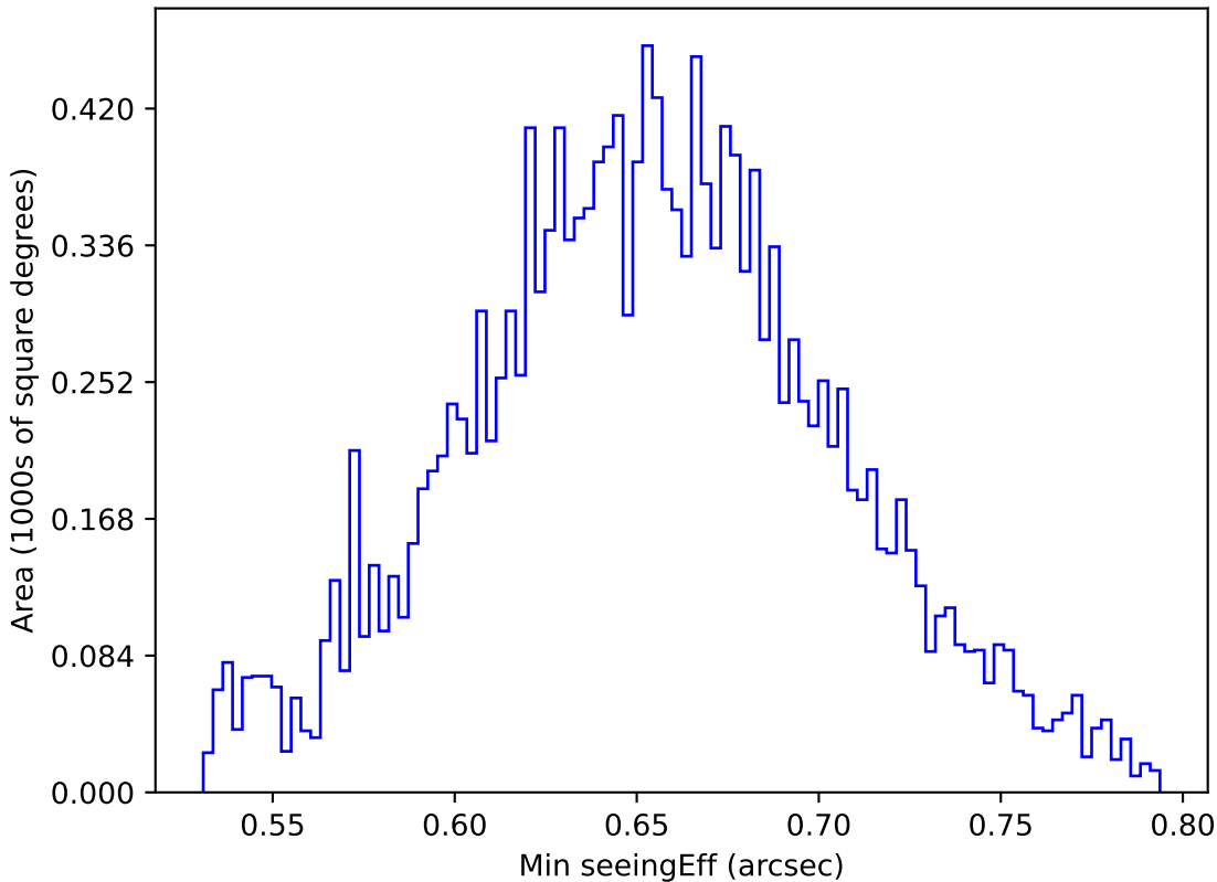
weather_cloudso0v3.4_10yrs WFD g band: Min seeingEff
