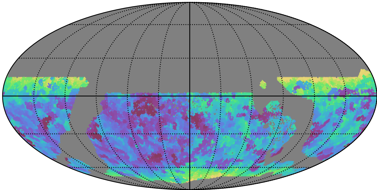
weather_cloudso0v3.4_10yrs WFD all bands: Min seeingEff
