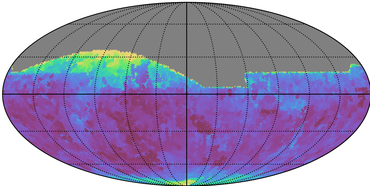
weather_cloudso0v3.4_10yrs All sky z band: Min seeingEff
