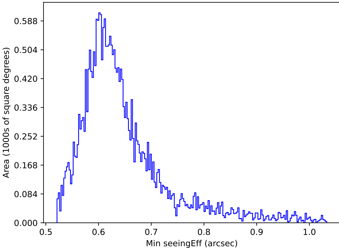
weather_cloudso0v3.4_10yrs All sky z band: Min seeingEff
