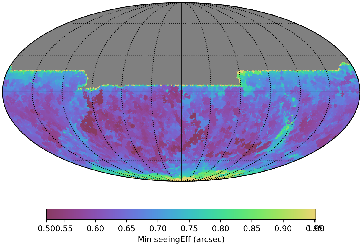
weather_cloudso0v3.4_10yrs All sky y band: Min seeingEff
