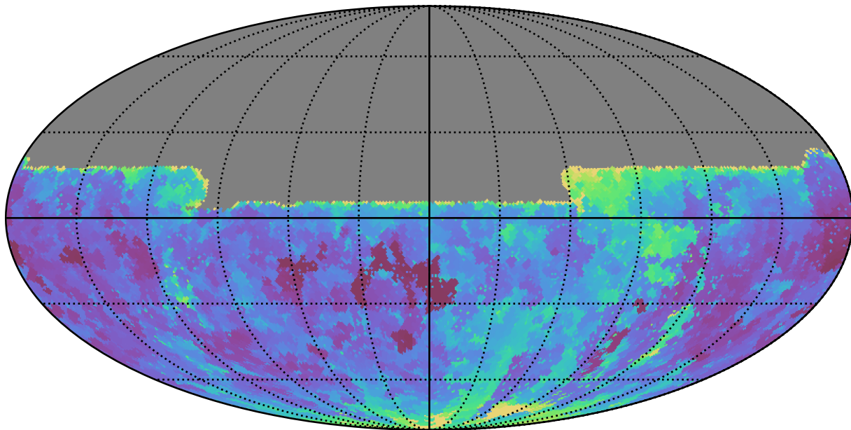
weather_cloudso0v3.4_10yrs All sky u band: Min seeingEff
