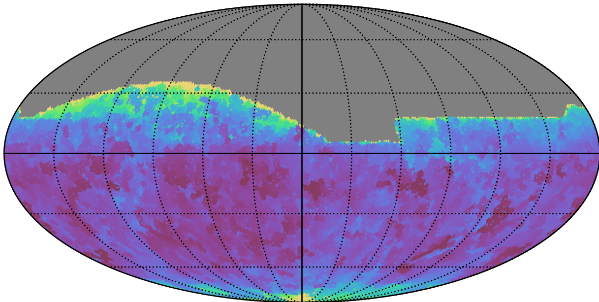
weather_cloudso0v3.4_10yrs All sky i band: Min seeingEff
