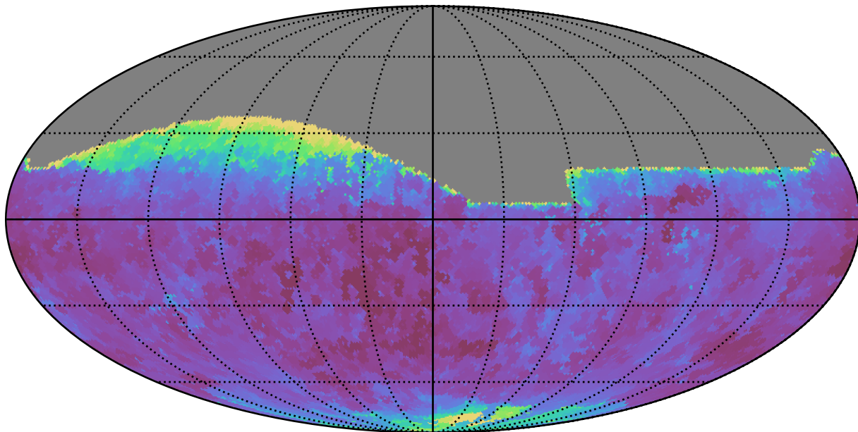
weather_cloudso0v3.4_10yrs All sky g band: Min seeingEff
