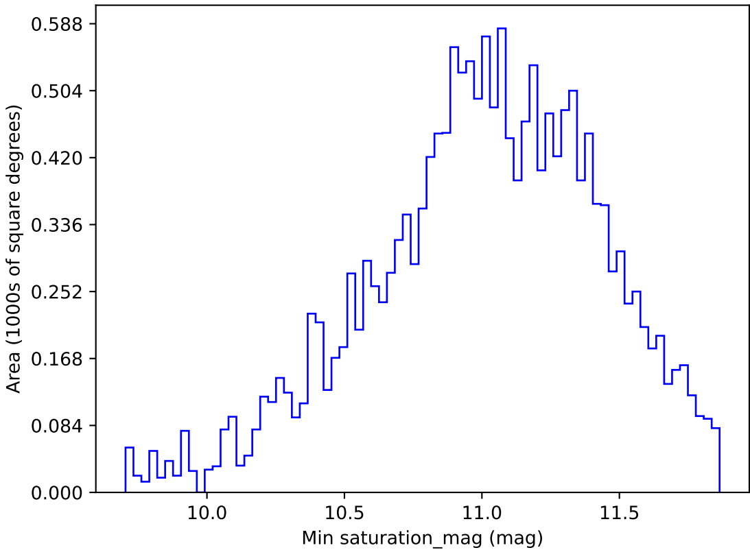
weather_cloudso0v3.4_10yrs WFD all bands: Min saturation_mag
