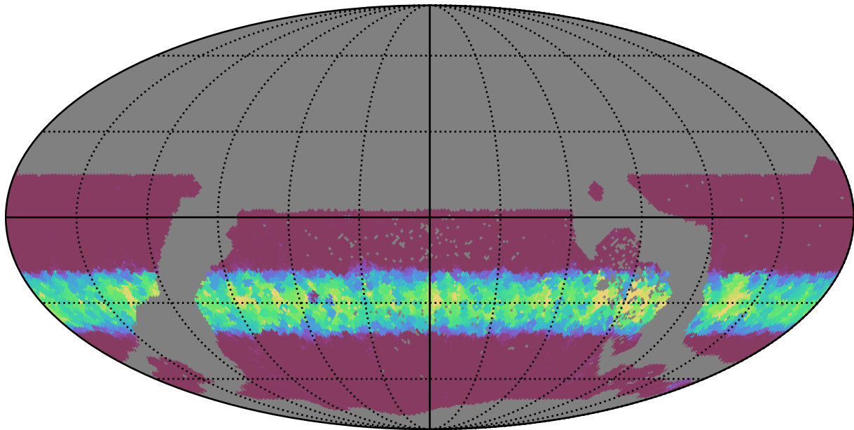
weather_cloudso0v3.4_10yrs WFD u band: Min normairmass
