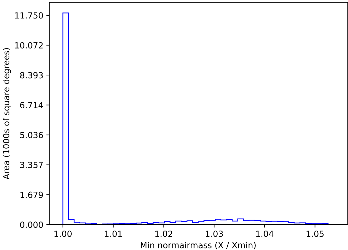
weather_cloudso0v3.4_10yrs WFD u band: Min normairmass
