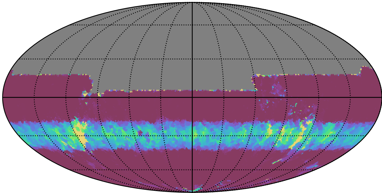
weather_cloudso0v3.4_10yrs All sky u band: Min normairmass
