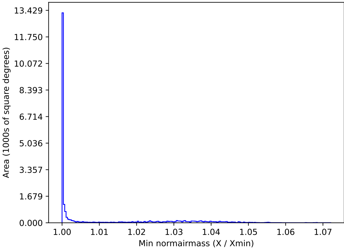
weather_cloudso0v3.4_10yrs All sky u band: Min normairmass
