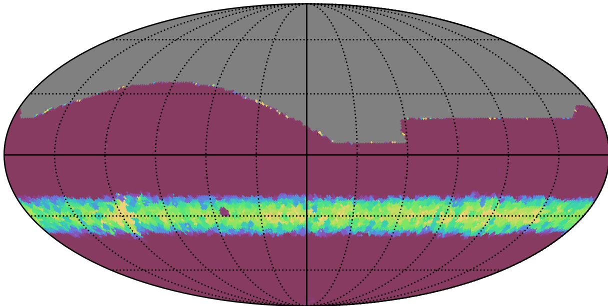
weather_cloudso0v3.4_10yrs All sky all bands: Min normairmass
