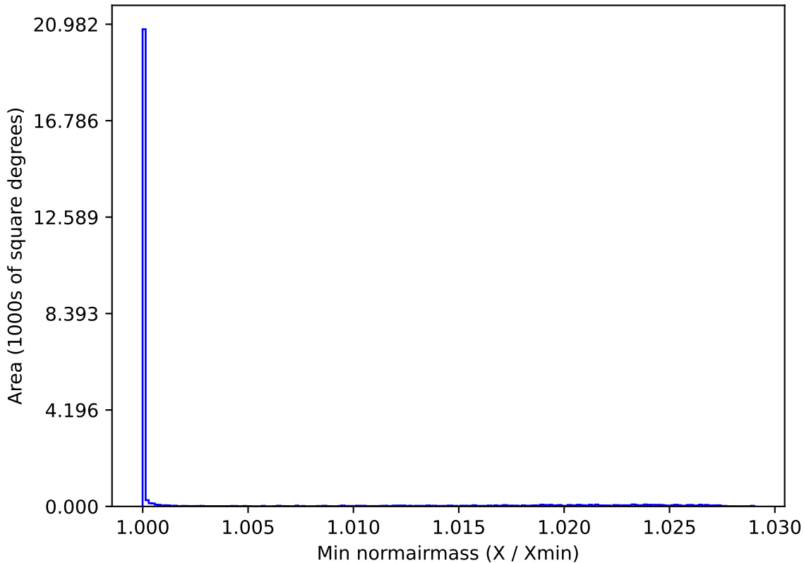
weather_cloudso0v3.4_10yrs All sky all bands: Min normairmass
