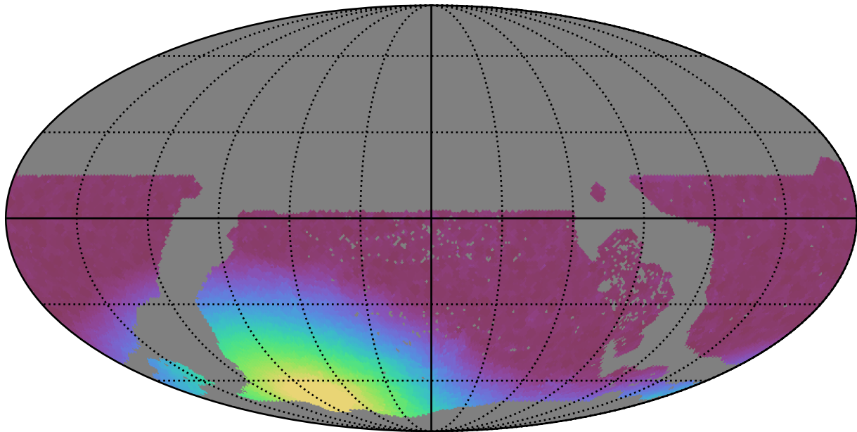
weather_cloudso0v3.4_10yrs WFD z band: Min moonDistance
