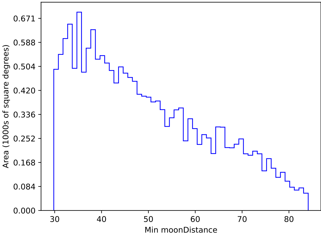
weather_cloudso0v3.4_10yrs WFD u band: Min moonDistance
