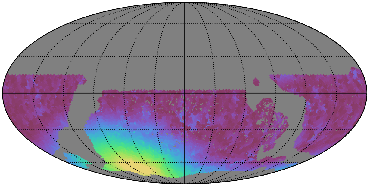
weather_cloudso0v3.4_10yrs WFD r band: Min moonDistance
