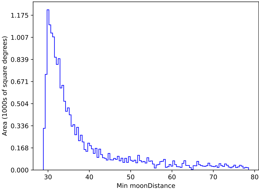
weather_cloudso0v3.4_10yrs WFD r band: Min moonDistance
