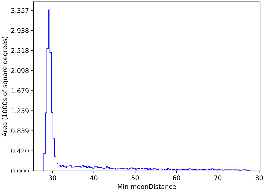
weather_cloudso0v3.4_10yrs WFD all bands: Min moonDistance
