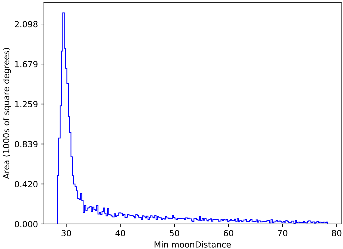
weather_cloudso0v3.4_10yrs All sky z band: Min moonDistance
