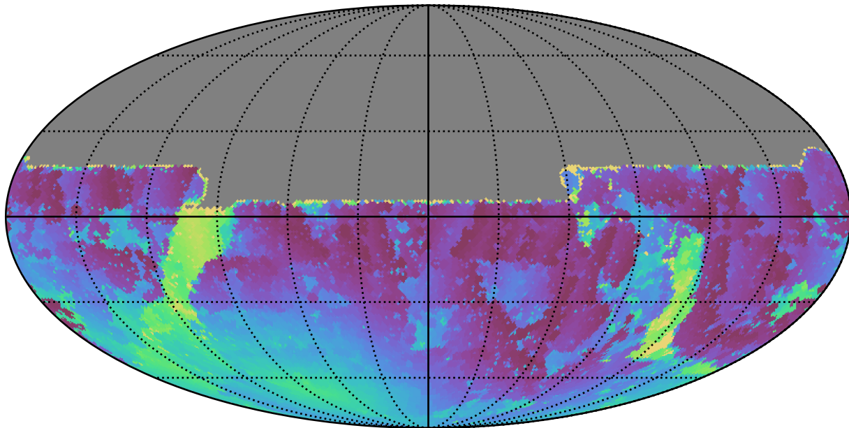
weather_cloudso0v3.4_10yrs All sky u band: Min moonDistance
