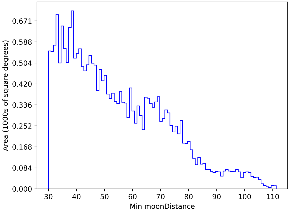
weather_cloudso0v3.4_10yrs All sky u band: Min moonDistance
