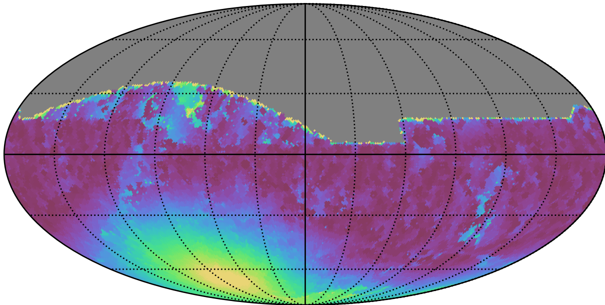
weather_cloudso0v3.4_10yrs All sky r band: Min moonDistance
