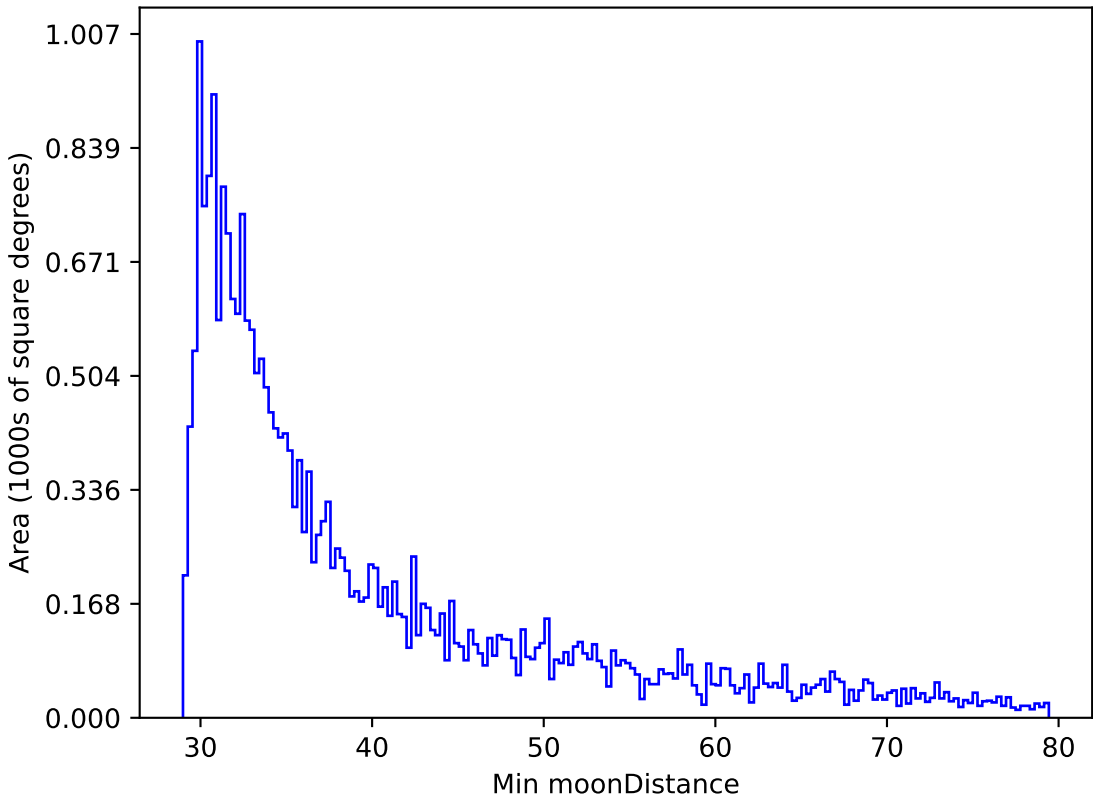
weather_cloudso0v3.4_10yrs All sky r band: Min moonDistance
