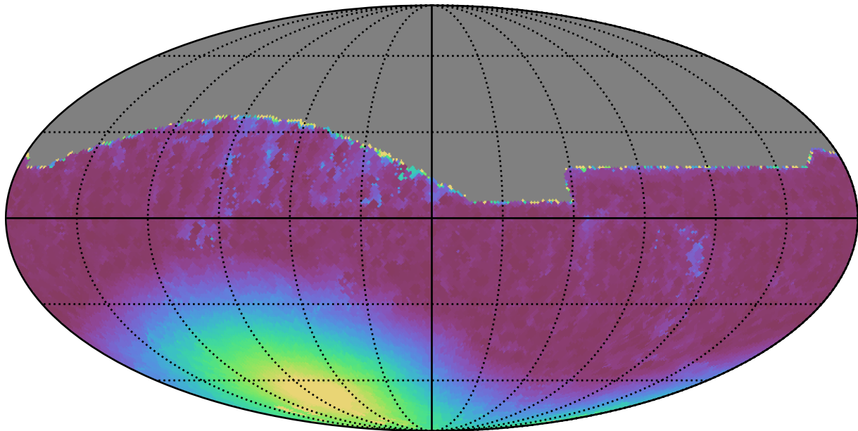
weather_cloudso0v3.4_10yrs All sky i band: Min moonDistance
