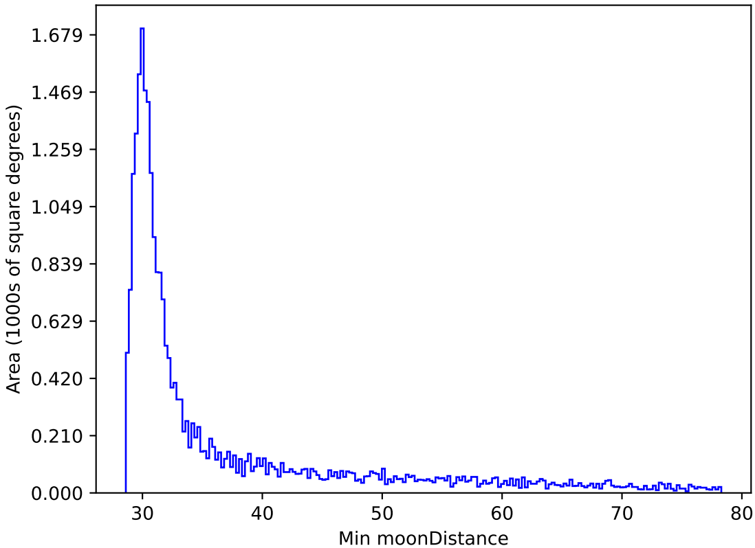
weather_cloudso0v3.4_10yrs All sky i band: Min moonDistance
