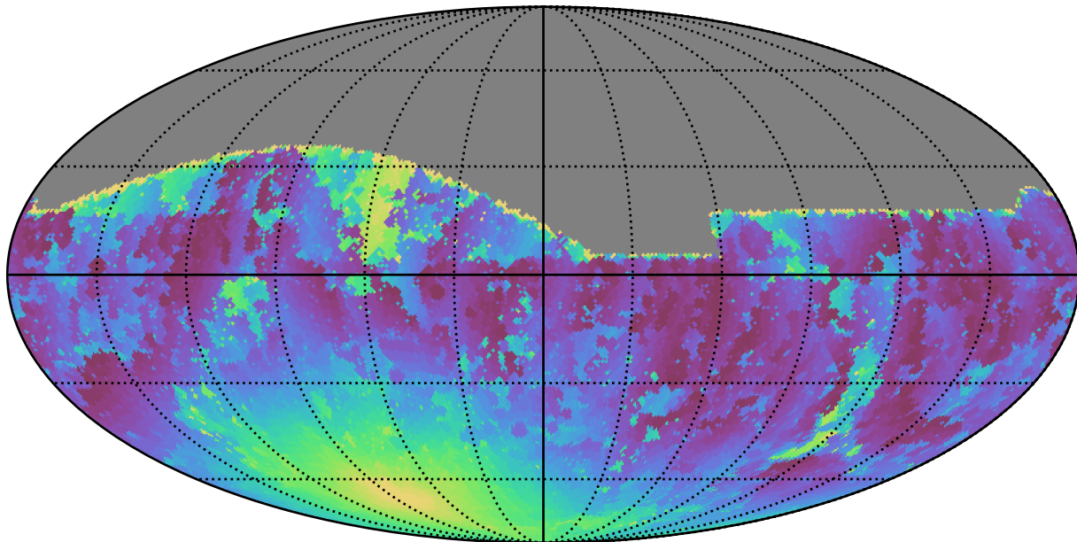
weather_cloudso0v3.4_10yrs All sky g band: Min moonDistance
