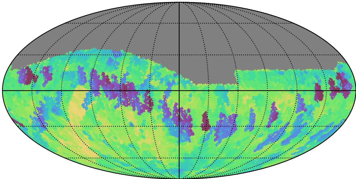
weather_cloudso0v3.4_10yrs Yr 1 z band: Min fiveSigmaDepth
