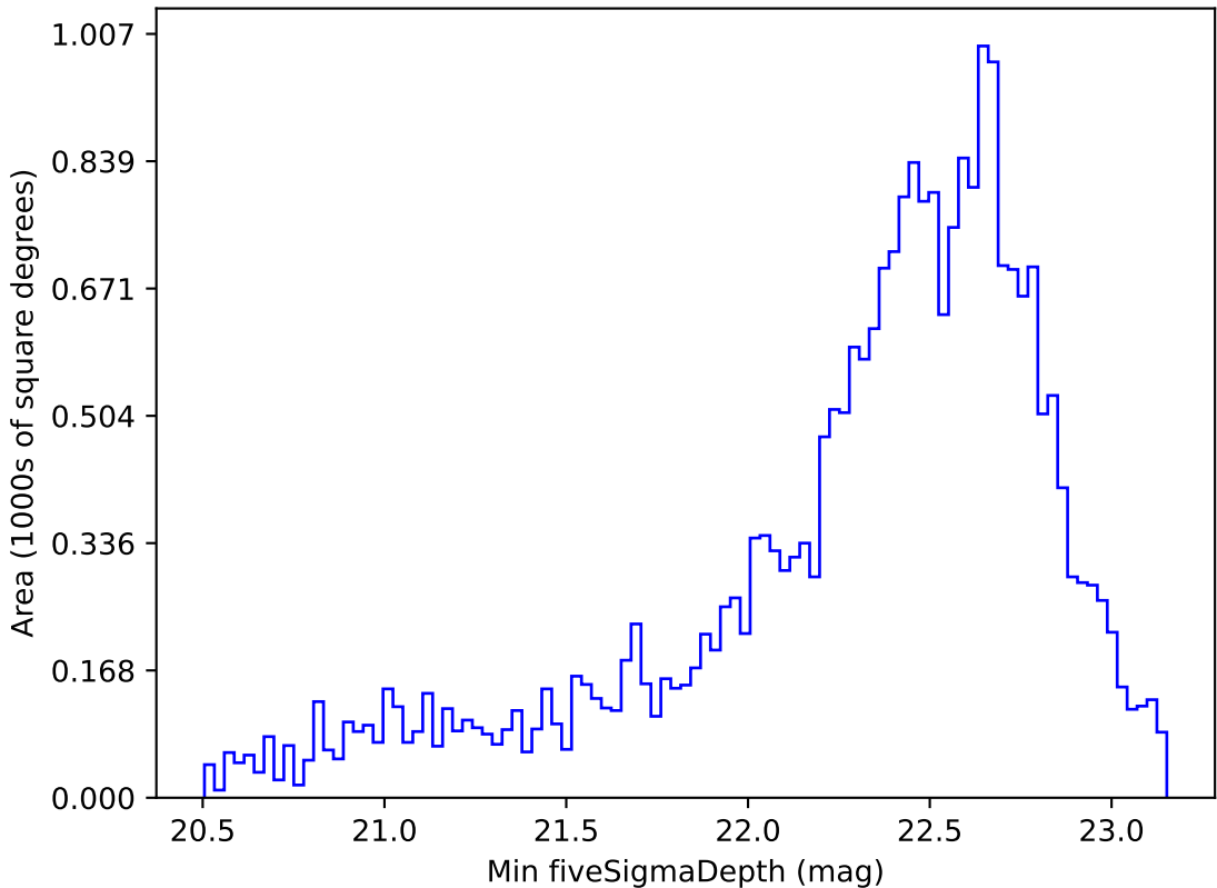
weather_cloudso0v3.4_10yrs Yr 1 z band: Min fiveSigmaDepth
