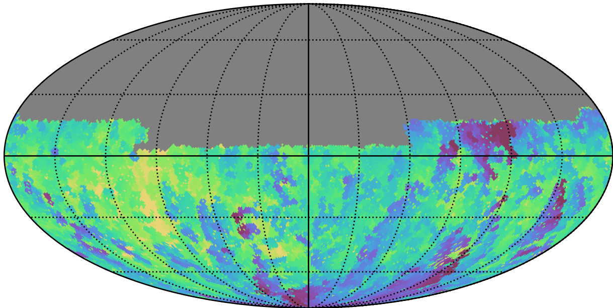
weather_cloudso0v3.4_10yrs Yr 1 u band: Min fiveSigmaDepth
