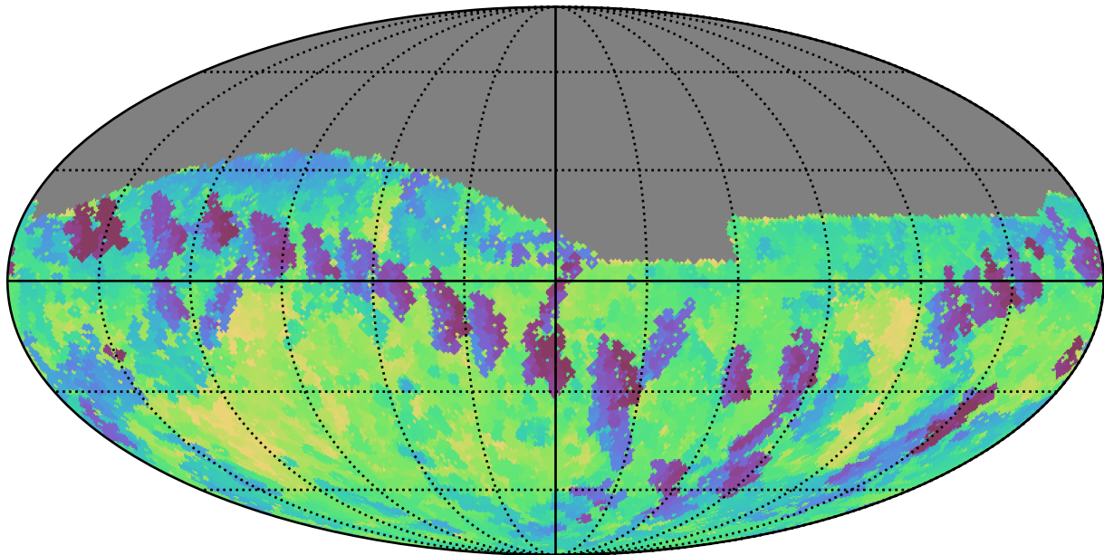
weather_cloudso0v3.4_10yrs Yr 1 i band: Min fiveSigmaDepth
