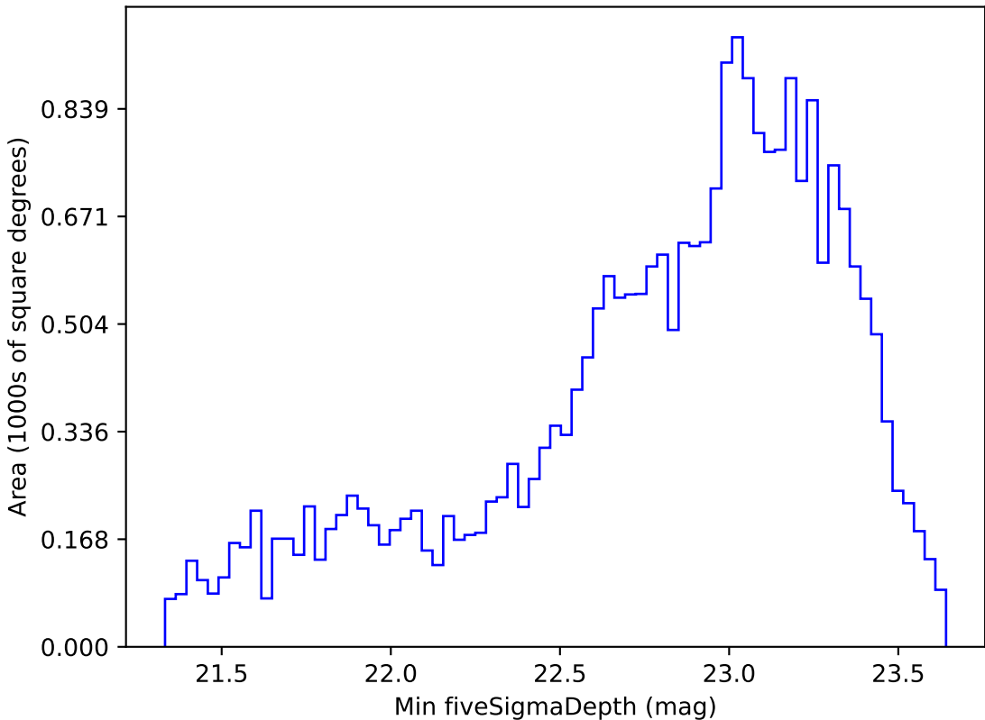
weather_cloudso0v3.4_10yrs Yr 1 i band: Min fiveSigmaDepth
