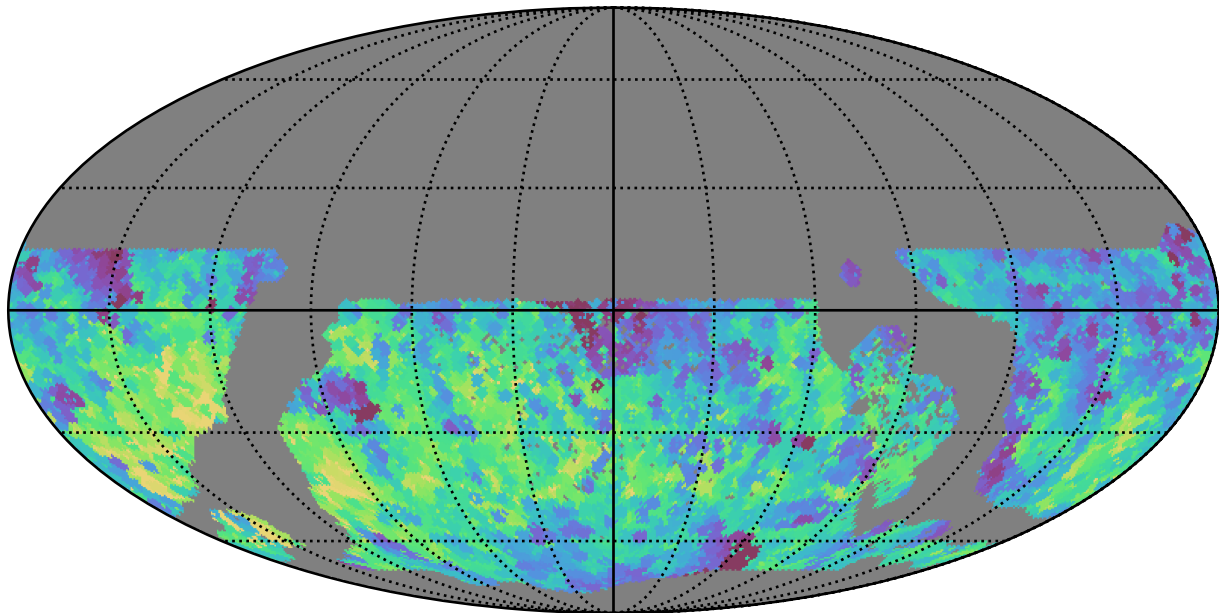
weather_cloudso0v3.4_10yrs WFD y band: Min fiveSigmaDepth
