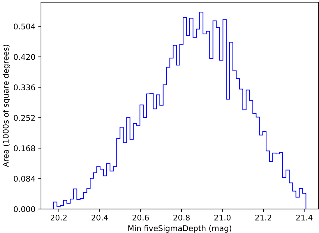
weather_cloudso0v3.4_10yrs WFD y band: Min fiveSigmaDepth
