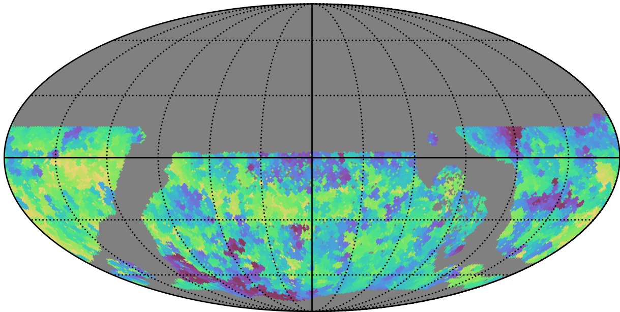
weather_cloudso0v3.4_10yrs WFD u band: Min fiveSigmaDepth
