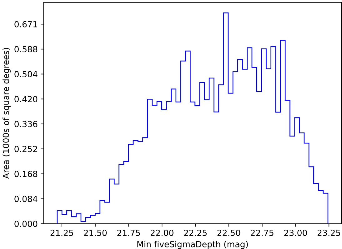
weather_cloudso0v3.4_10yrs WFD r band: Min fiveSigmaDepth
