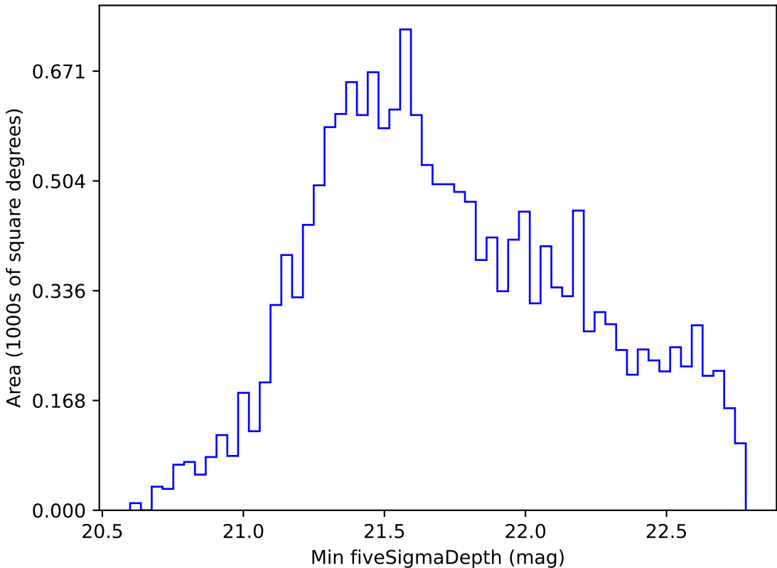
weather_cloudso0v3.4_10yrs WFD i band: Min fiveSigmaDepth
