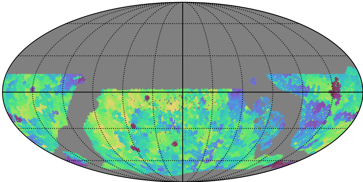
weather_cloudso0v3.4_10yrs WFD g band: Min fiveSigmaDepth
