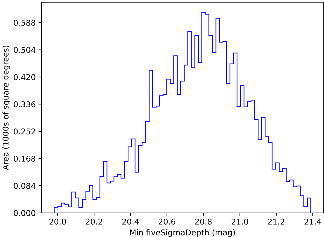
weather_cloudso0v3.4_10yrs WFD all bands: Min fiveSigmaDepth
