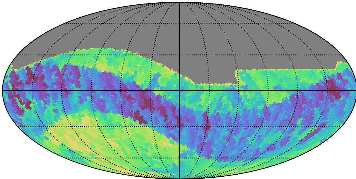
weather_cloudso0v3.4_10yrs All sky z band: Min fiveSigmaDepth
