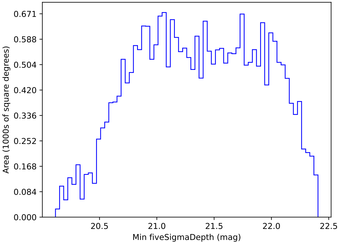
weather_cloudso0v3.4_10yrs All sky z band: Min fiveSigmaDepth
