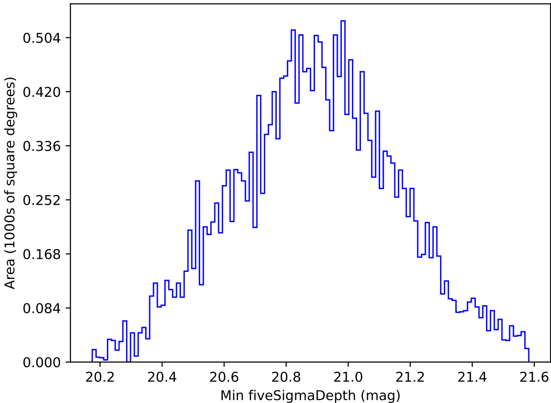
weather_cloudso0v3.4_10yrs All sky y band: Min fiveSigmaDepth
