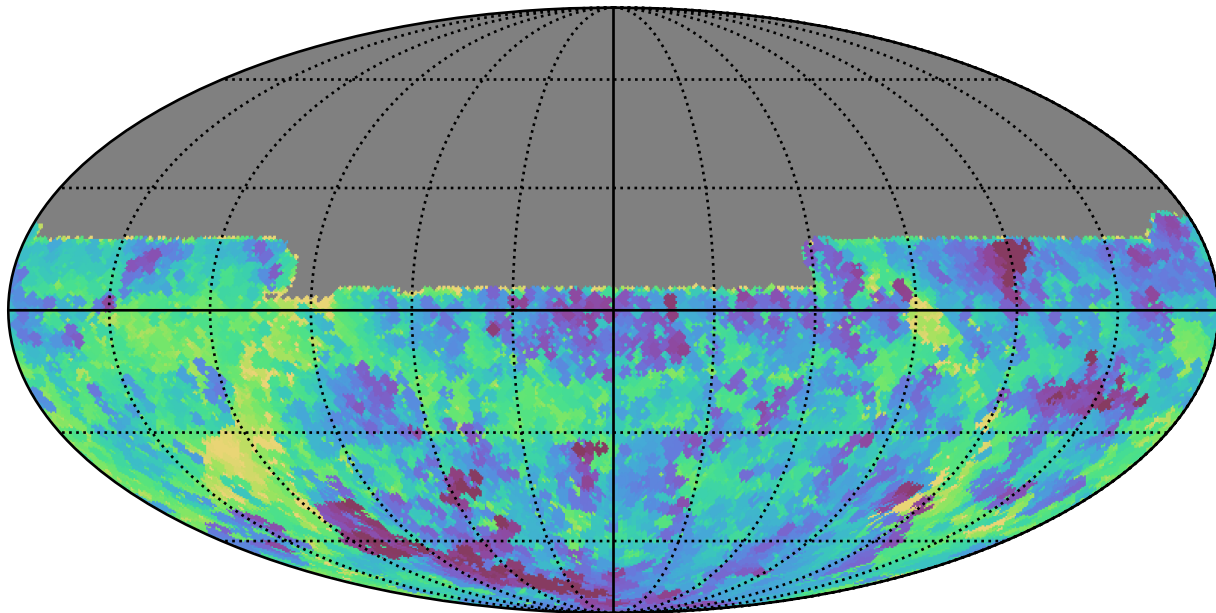
weather_cloudso0v3.4_10yrs All sky u band: Min fiveSigmaDepth
