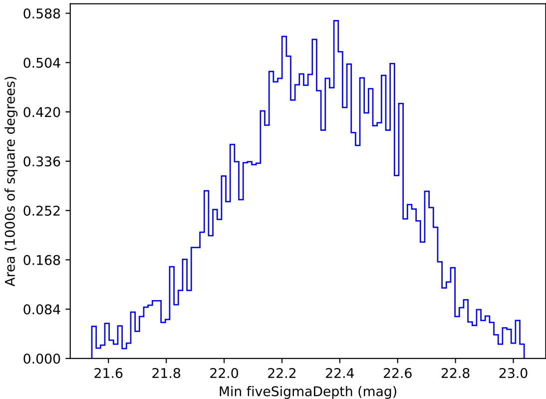
weather_cloudso0v3.4_10yrs All sky u band: Min fiveSigmaDepth
