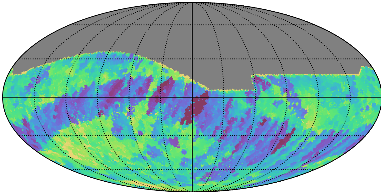
weather_cloudso0v3.4_10yrs All sky r band: Min fiveSigmaDepth
