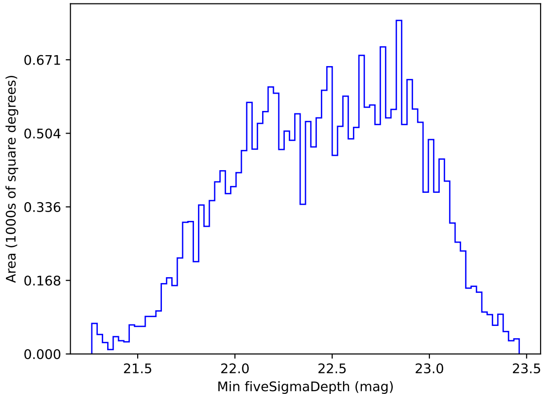
weather_cloudso0v3.4_10yrs All sky r band: Min fiveSigmaDepth
