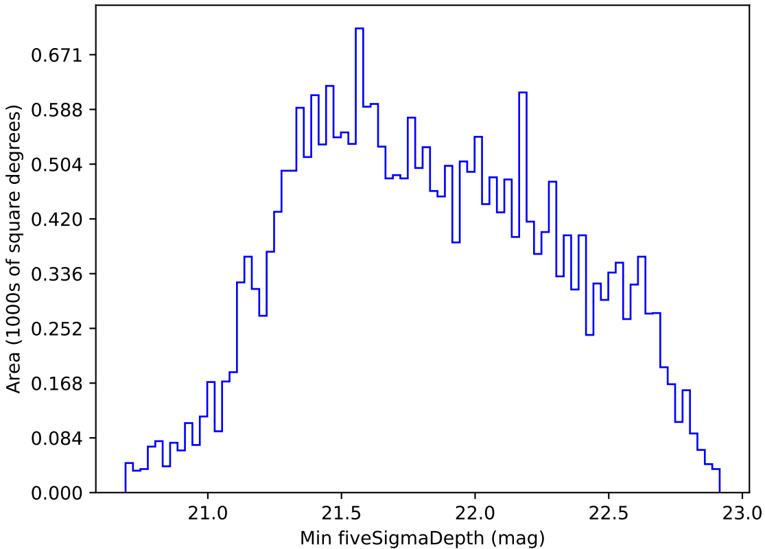
weather_cloudso0v3.4_10yrs All sky i band: Min fiveSigmaDepth
