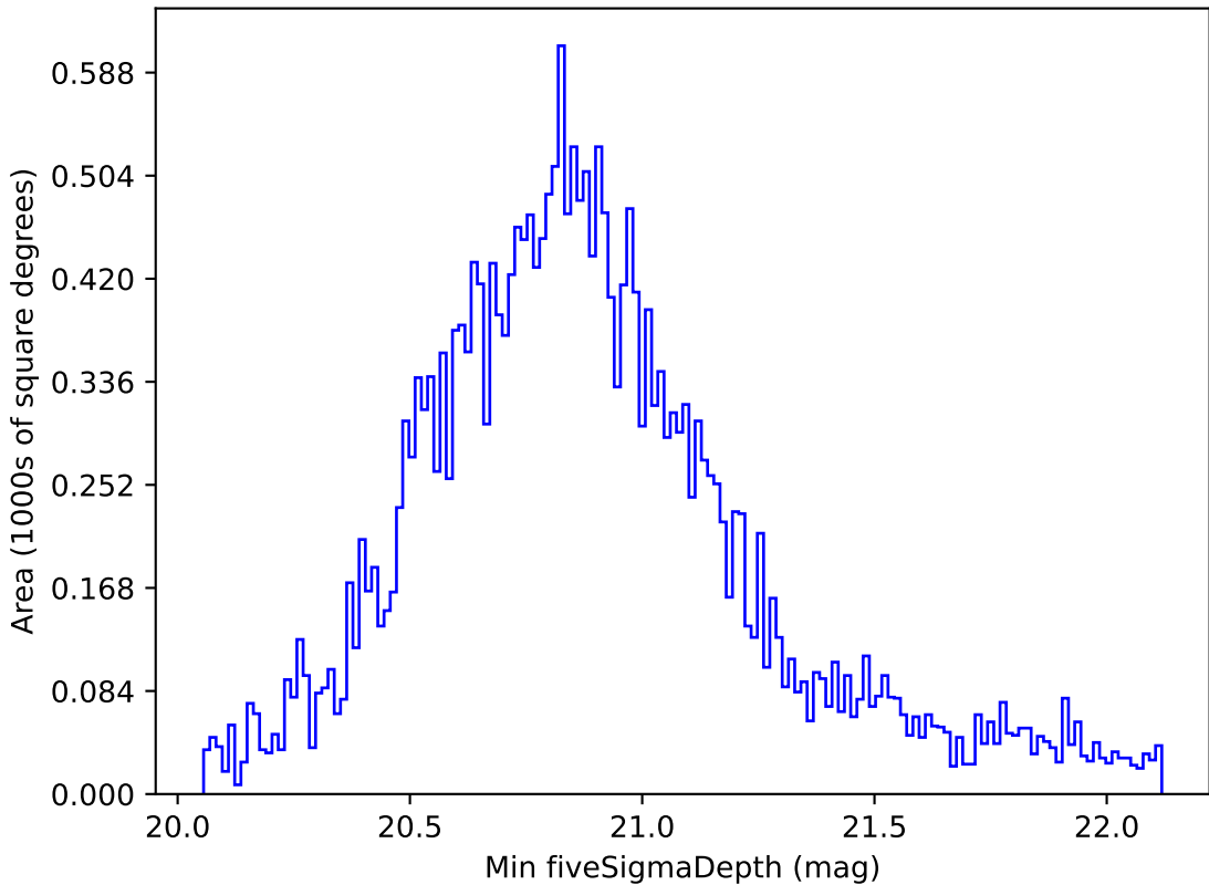
weather_cloudso0v3.4_10yrs All sky all bands: Min fiveSigmaDepth
