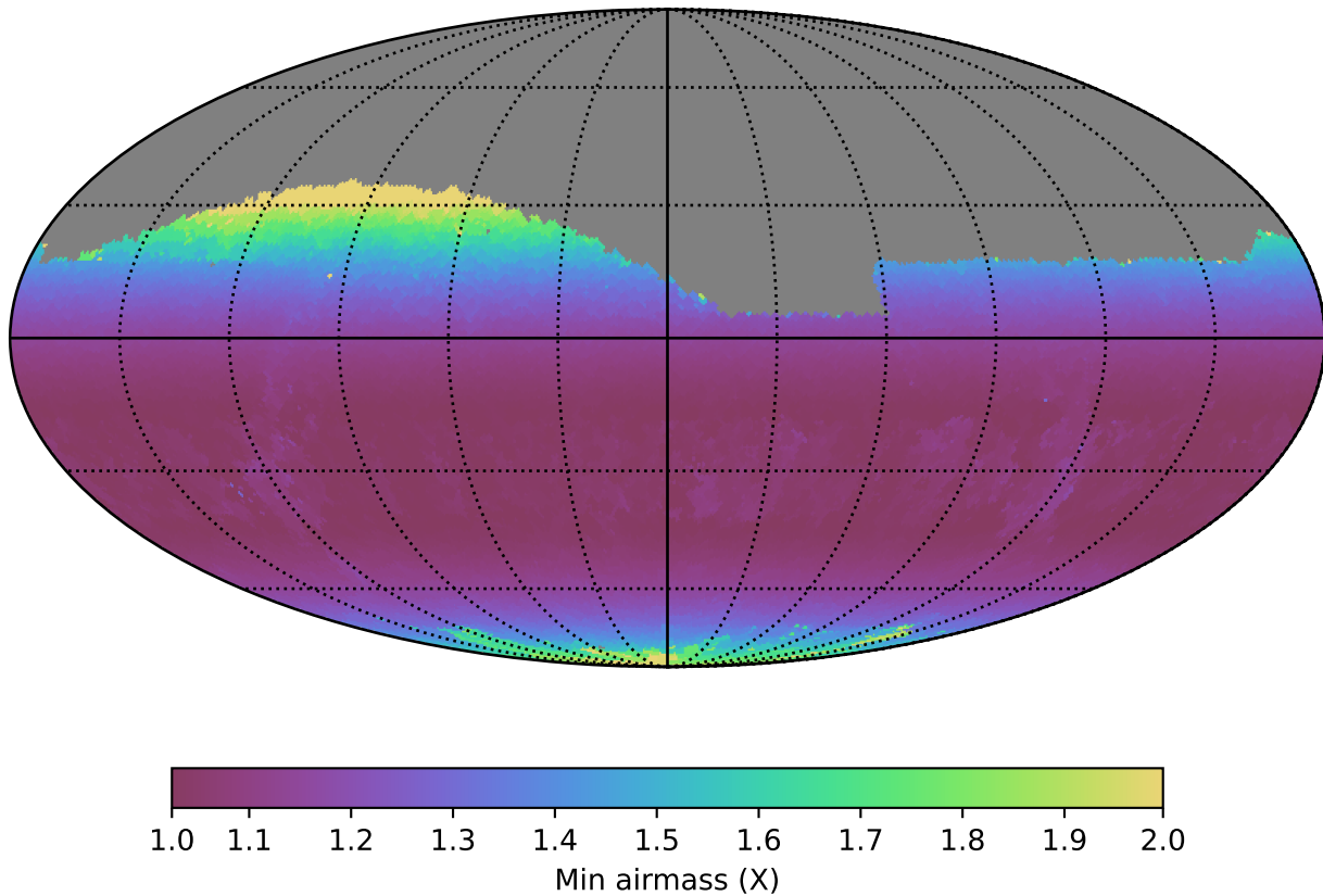
weather_cloudso0v3.4_10yrs Yr 1 z band: Min airmass
